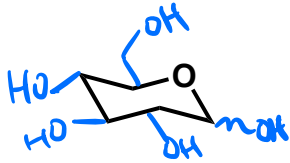
Glc
